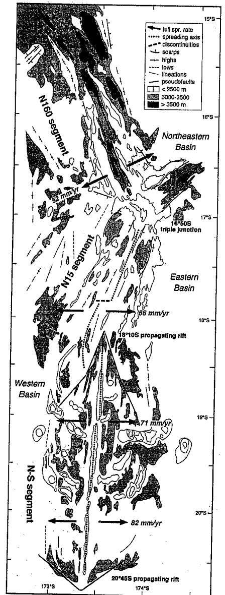
Fig. 5. Geodynamic sketch of the Central Spreading Ridge (North Fiji Basin). Spreading rates are from magnetic anomalies. young spreading areas, like the Central Bransfield Basin and Tripartite Ridge respectively, suggests a regular spacing
