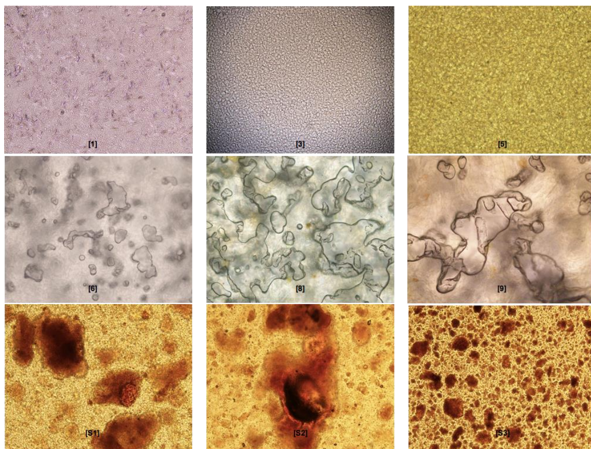
Figure 7. Transmitted Light Microscope micrographs for examined biogenic grease samples (window sizes of 683.5 \mu\text{m} \times 536 \mu\text{m} ) [19].
