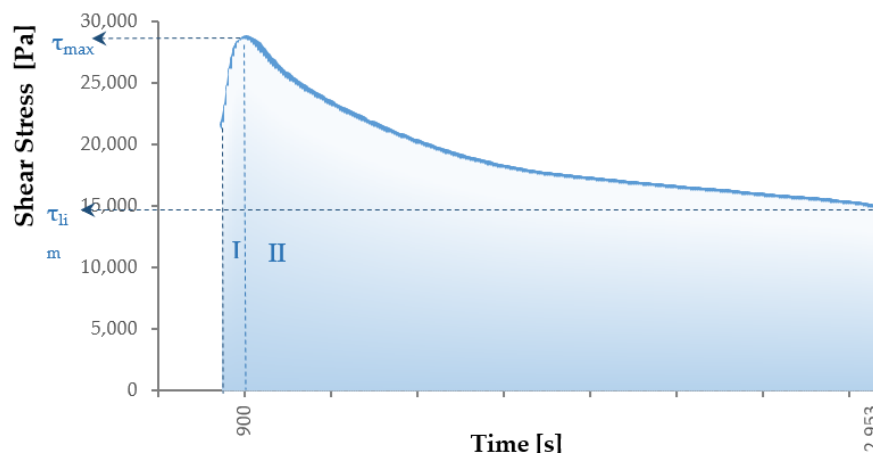
Figure 1. Example of a stress vs. time curve obtained in rotational transient flow tests.
