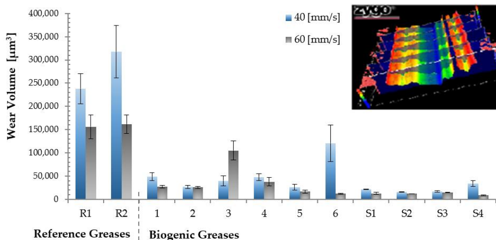
Figure 4. Wear volume in steel disc (Wear path s_R = 80 m).
