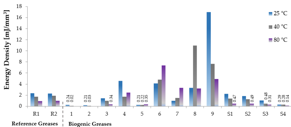
Figure 6. Energy densities ( e_{rheo} ) determined by integration of the shear stress vs. time plots at 25 °C, 40 °C, and 80 °C.
