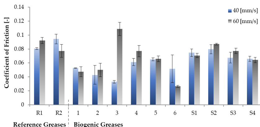
Figure 2. Friction coefficients determined in a steel ball-on-steel disc configuration (wear path s_R = 80 \text{ m} ).
