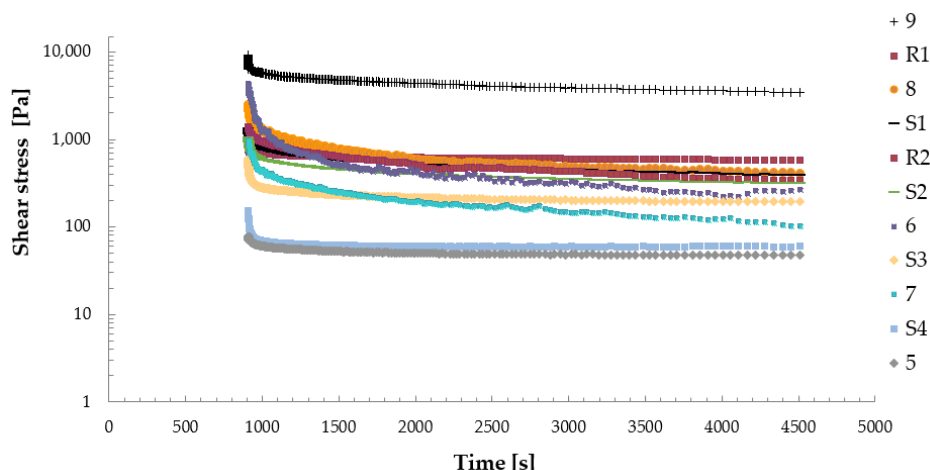
Figure 5. Transient flow curves for selected model grease samples at 25 °C.
