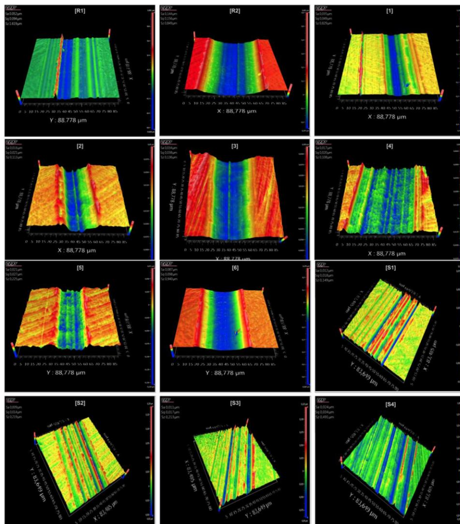
Figure 3. Profilometric pictures obtained from the steel discs as a function of the grease used as lubricants (window sizes of 88,778 \mu\text{m} \times 88,778 \mu\text{m} and 83,485 \mu\text{m} \times 83,649 \mu\text{m} ).
