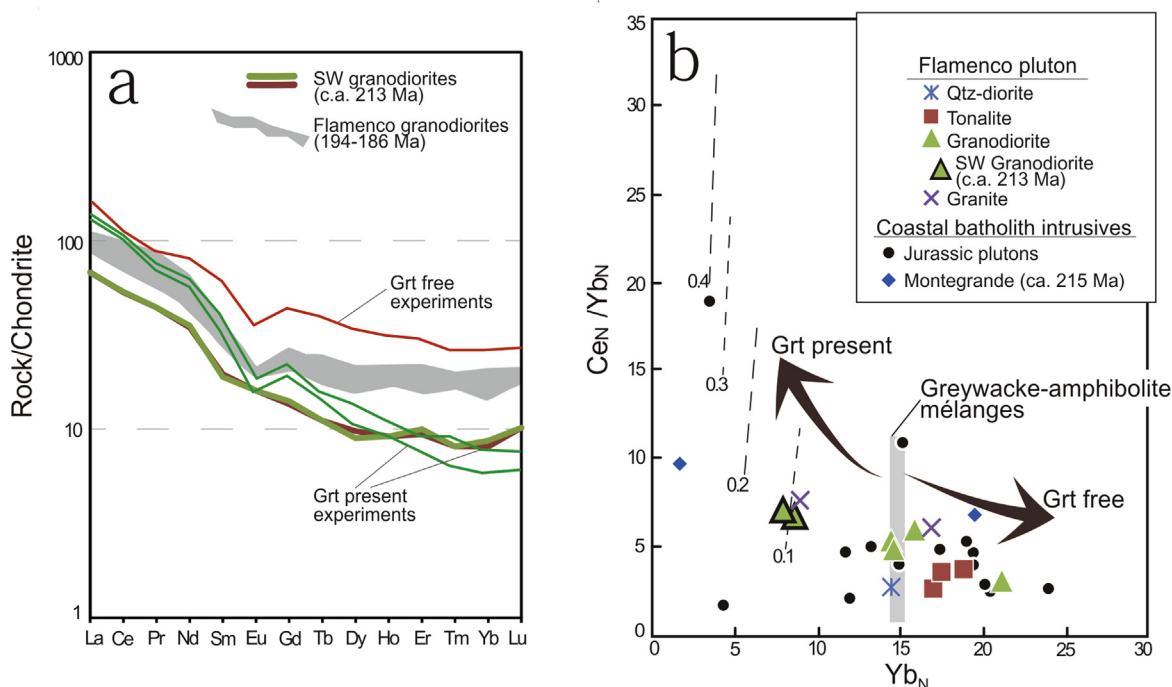
Figure 12. (a) Chondrite-normalized (Nakamura, 1974) REE diagram for the early SW leucocratic granodiorites (ca. 213 Ma) and for the younger studied granodiorites (194–186 Ma) from the Flamenco pluton. REE patterns obtained for Grt-free and Grt-present experimental assemblages in subducted mélangé (aprox. andesitic) compositions (Castro et al., 2010) are plotted for comparison. (b) Ce N /Yb N vs. Yb N diagram showing the geochemical differences between the SW leucocratic granodiorites and the rest of the samples of the Flamenco pluton. Limarí and Papudo-Quintero Jurassic intrusive complexes (Parada et al., 1999) and Montegrande granites (Coloma et al., 2017) are plotted for comparison. The Grt-free and Grt-present fields are experimentally calculated for a greywacke-amphibolite mixed source (Castro et al., 2010) depicting the “adakitic” trends (high Ce N /Yb N and low Yb N contents). Dashed lines represent the Grt wt.% in the experimental assemblages.
