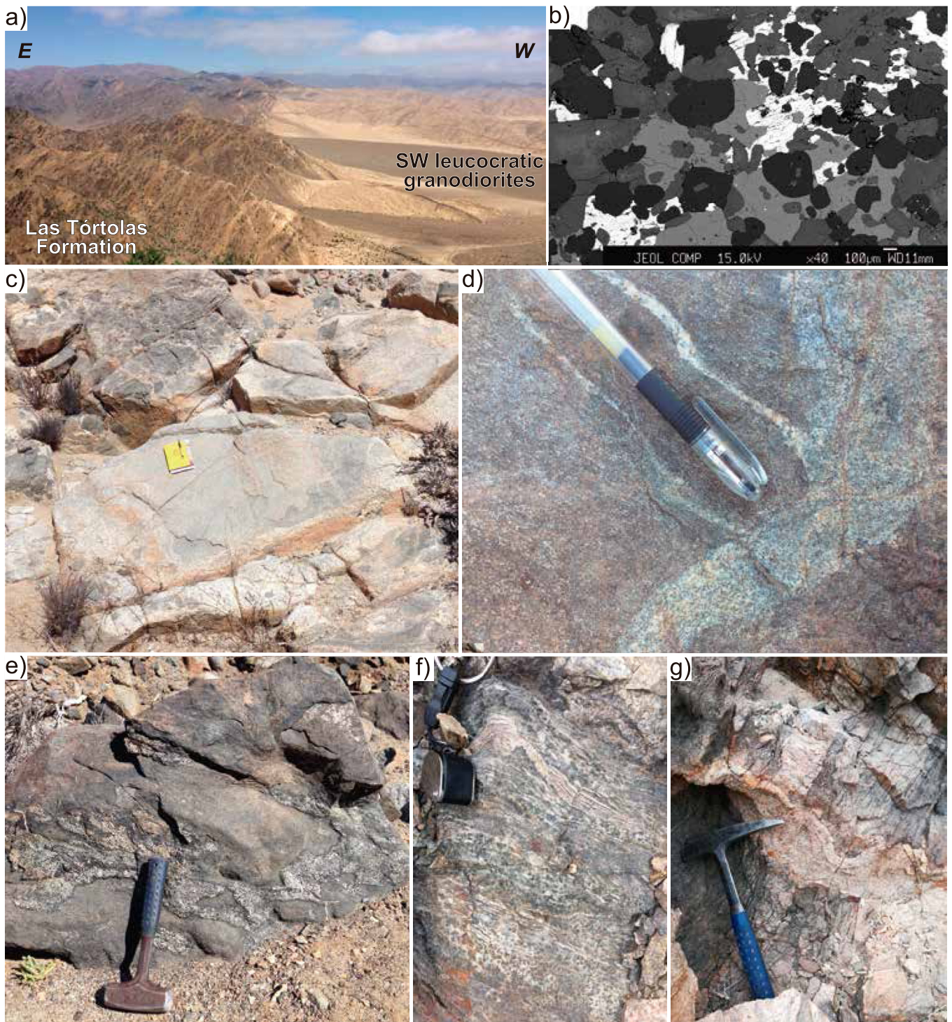
Figure 2. (a) View (to the south) of the southern contact of the Flamenco pluton where the Las Tórtolas Formation are located above the SW leucocratic granodiorites. (b) Mesocratic granodiorites located between the NW Qtz-diorites and tonalites and NW tonalites and granodiorites (yellow line in Fig. 1c) present granulitic recrystallization textures. These rocks show Hbl-Pl-Qtz triple junctions and poikiloblastic Kfs. (c) Mingling areas between gabbros and tonalites located close to the shear zone at the eastern area of the Flamenco pluton (Fig. 1c). Where the gabbroic enclaves are affected by the shear zone, subsolidus fabrics (parallel to the pen in the image) are observed in these gabbros (d). (e–g) Las Tórtolas Formation volcanic and sedimentary rocks located in the contact metamorphic aureole of the Flamenco pluton. Recrystallized basalts at the northern contact (e) and Crd-schists (f) to the south present the highest metamorphic grade in the host metasedimentary rocks. There, some thick leucocratic veins and melanosomes (g) characterize a narrow migmatitic domain.
