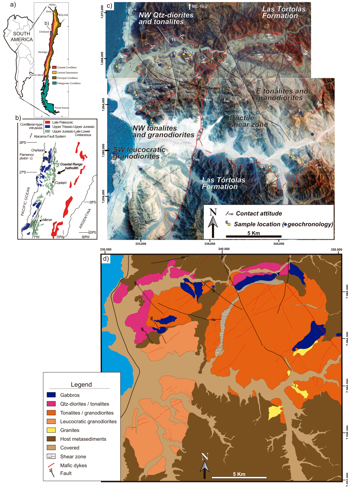
Figure 1. (a) Major morphological features of the Andean cordillera in Chile (modified from Charrier et al., 2007). (b) Sketch of a section of the west margin of Southamerica from 29°S to 26°S showing the distribution of the Cordilleran-type magmatism between the late Paleozoic to the late Lower Cretaceous (Coastal Range batholith) (modified from Charrier et al., 2007; Maksiyev et al., 2014). Major faults that comprise the Atacama Fault System are indicated. (c) Satellite image of the Flamenco pluton. The contacts with the host metasediments (red lines), the main intrusive units and some structural features are pointed over the image. The locations of the samples employed in the geochemical and geochronological study are indicated. (d) Geological map of the Flamenco pluton with the main mesoscopic petrological units.
