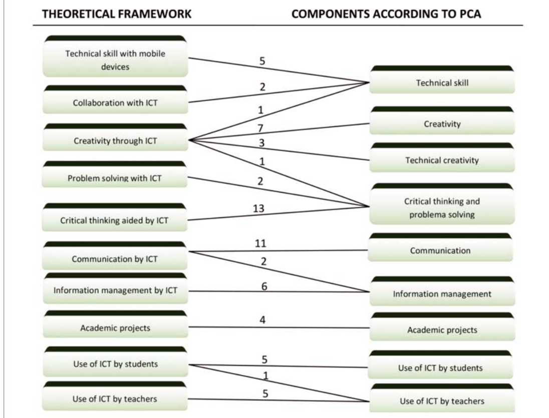
Figure 2. Relationship of items between the categories of the theoretical framework and PCA results
