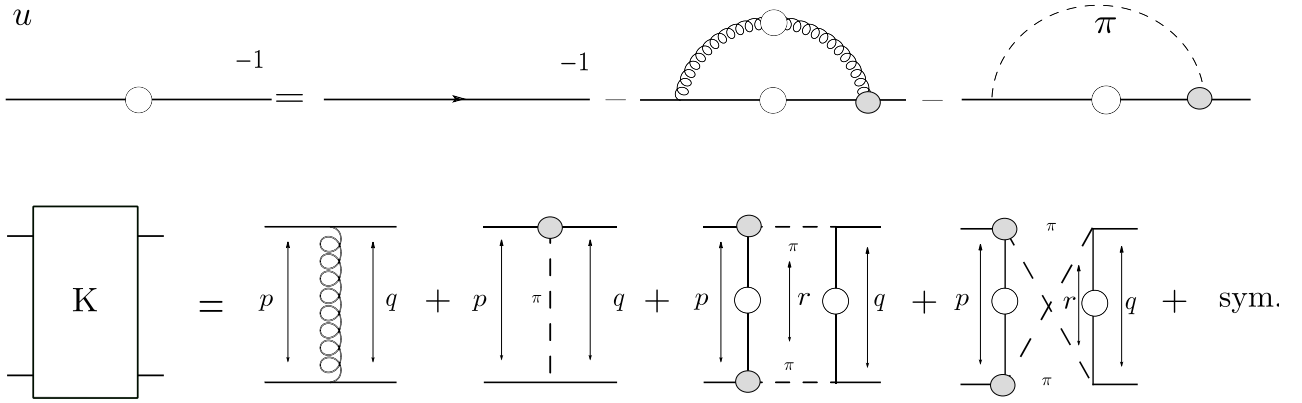
Fig. A1. Truncations employed for the BSE interaction kernel K (lower diagrams) and the quark SDE one (upper diagrams). In the lower panel, the diagrams on the right-hand side correspond to the RL, pion exchange, and the s -channel together with the u -channel pion decay contributions, respectively.
