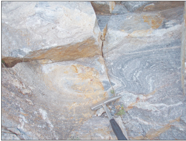
FIGURE 9. Elliptical cross-section of a sheath fold showing a high Y-Z aspect ratio. Marble Formation, Sierra Blanca (Western Betics).
