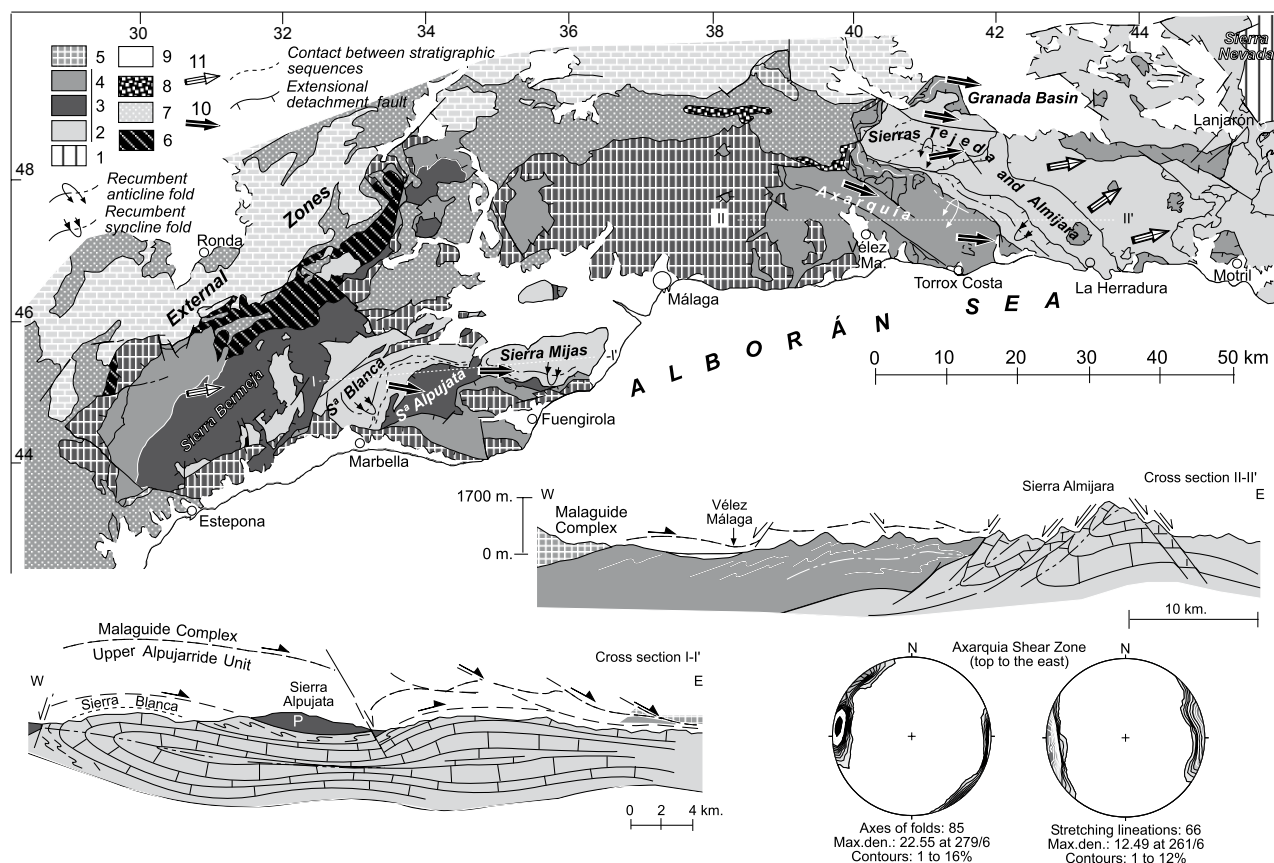
FIGURE 2. Top-to-the-east extensional shear zone in Western and Central Alpujarras Domains. 1) Nevado-Filabride Complex. 2) Lower and Intermediate Alpujarras Extensional units. 3) Peridotites. 4) Upper Alpujarras Extensional Unit. 5) Maláguide Complex. 6) Dorsalian units. 7) Flysch units. 8) Viñuela and related units. 9) Neogene and Plio-Quaternary sediments. 10) Stretching lineation and shear sense. 11) Stretching lineation and shear sense (after Simancas and Campos, 1993; Balanyá et al. , 1997; Rossetti et al. , 2005). Axial-traces of large recumbent folds and simplified sections across them in the areas of the Sierra Blanca-Sierra de Mijas in the western Betics and the Axarquía region are also represented.
