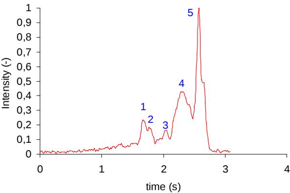
Figure 4. Light curve (relative intensity vs. time).
