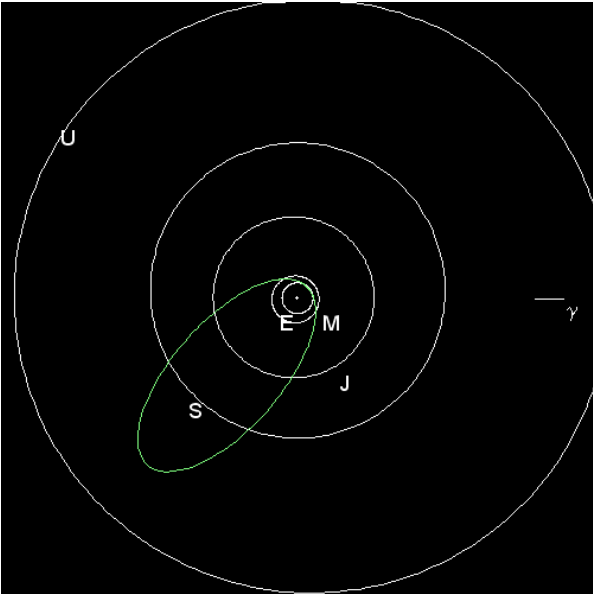
Figure 3. Projection on the ecliptic plane of the orbit of the parent meteoroid.
