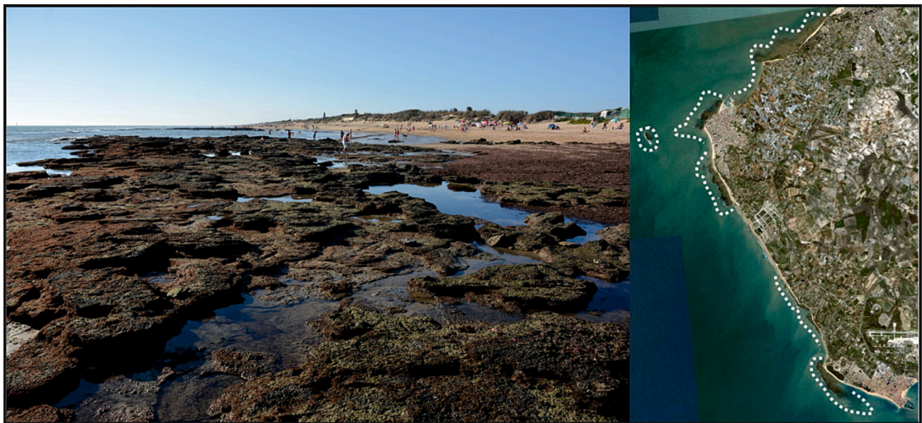
Fig. 5. Left: A close view of the shore platform south of Chipiona city. Right: Extension of the shore platform in the study zone.
