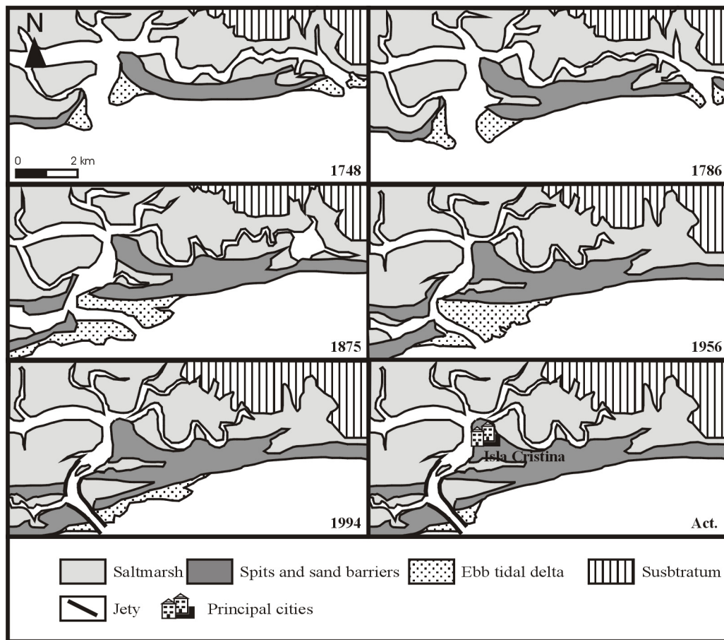
Fig. 10.- Coastal evolution of the Carreras tidal channel sector from 1748 to present (Morales et al. , 1997, modified).
