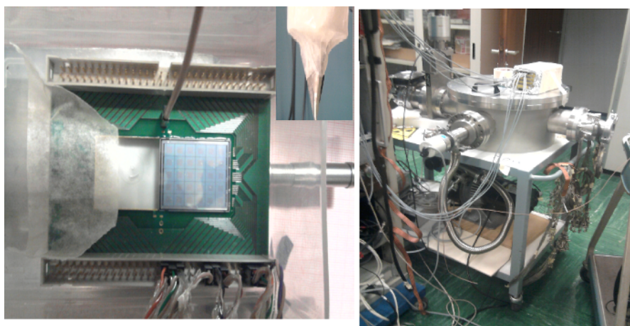
Figure 1. On the Left, a prototype of the TRACE pad detector on a micrometer scanning system is visible. The steel cone used as a collimator is also presented in the inset. On the right, the experimental setup, with the chamber and the preamplifier in foreground.
