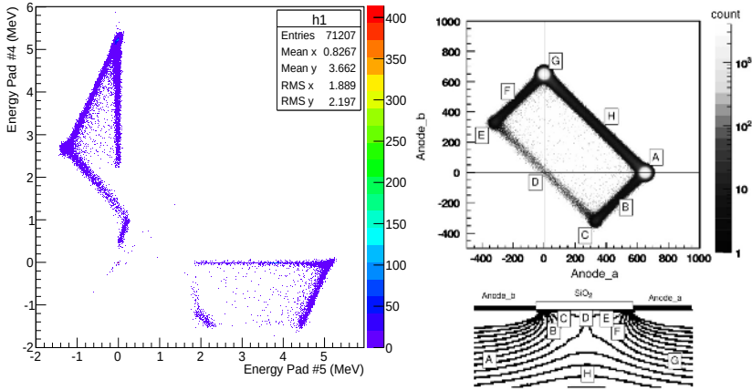
Figure 3. Energy correlation matrix among two neighboring pads. The matrix shows two important zones: the zone of the maximum energy for each pad, recognizable from the scale intensity and the charge-sharing zone, the lines almost parallel to the first bisector. On the top right, the simulation [6] of the correlation matrix between the energy of two neighboring pads. On the bottom right, the calculation of the electric field, where the four regions and vertices of the correlation matrix are spot. The presence of points along the X and Y axis, at an energy lower than the alpha peak, is likely to be ascribed to a charge loss in the inter-pad region.
