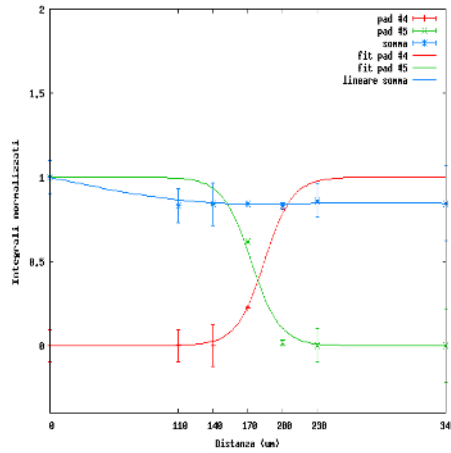
Figure 2. Normalized intensity as a function of the position during the scan. The zero was chosen arbitrarily to have the collimating source in the center of a pad. The lines are obtained by a Fermi-Dirac function.
