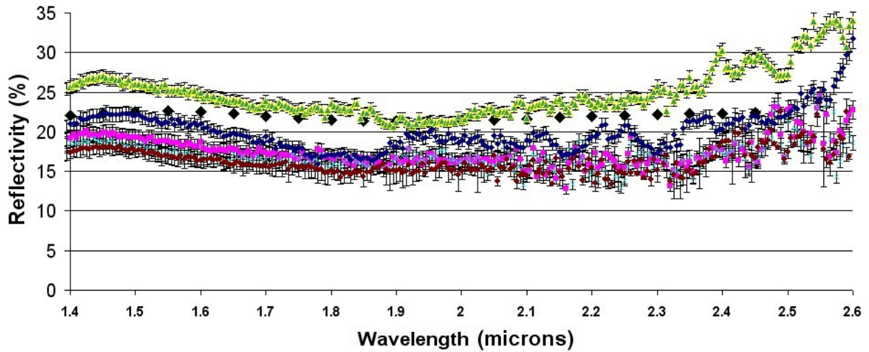
Figure 1b. Spectra of ordinary chondrites in the 1.4 to 2.6 \mu\text{m} range (see Fig. 1a caption for additional details).
