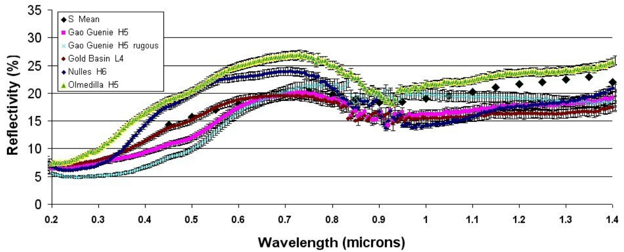
Figure 1a. UV-visible-near IR spectra of ordinary chondrites analyzed in this study in the 0.2 to 1.4 \mu\text{m} range (see Table 1 for additional details). 1\sigma error bars are included to take into account the scattering among the measurements.
