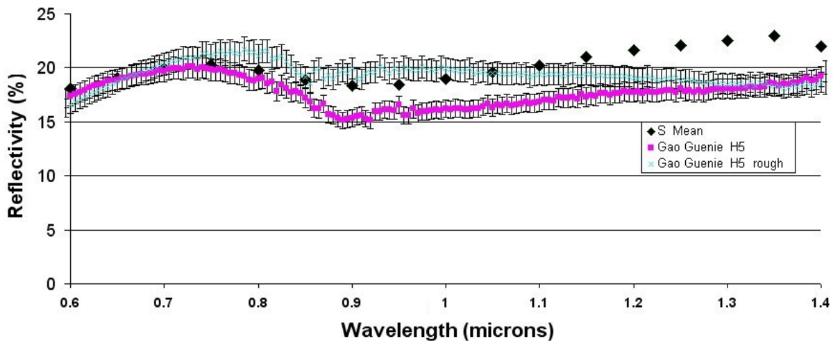
Figure 2. Main differences in the reflectance spectrum of the H5 ordinary chondrite Gao Guenie for a polished and a rugous section in the 0.6 to 1.4 microns range. Note that the rough sample tends to fit better the S mean spectrum below 1.1 \mu\text{m} .
