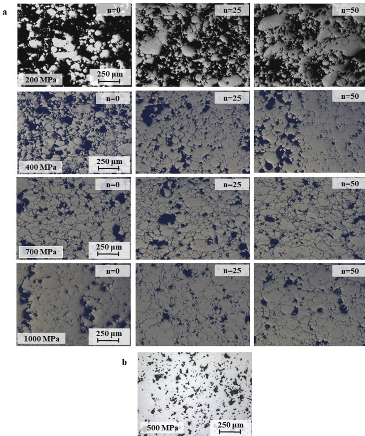
Fig. 6. Micrographs showing the porosity distribution for (a) different number of discharges with green compaction pressures of 200, 400, 700 and 1000 MPa; (b) the conventionally sintered compact. (For interpretation of the references to colour in this figure legend, the reader is referred to the web version of this article.)
