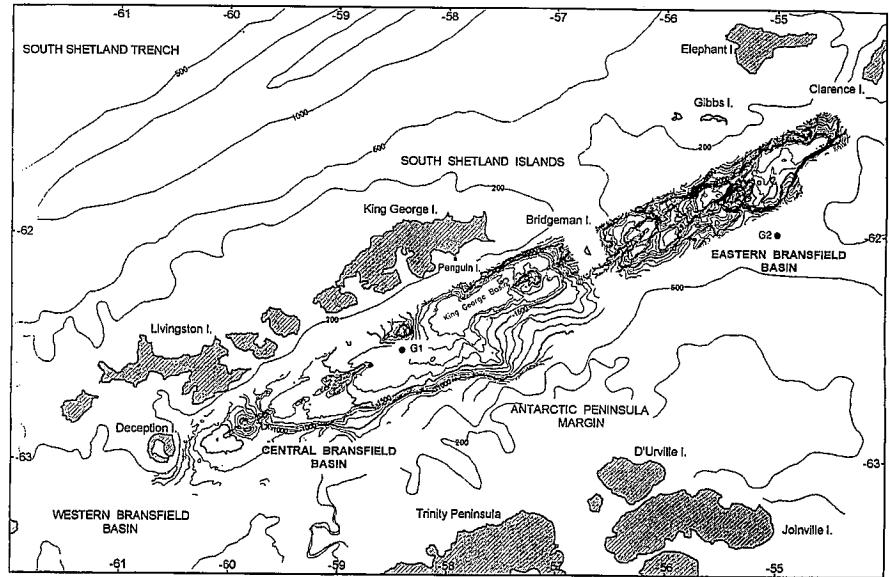
Fig.1. Bathymetric chart of the Bransfield Basin with the location of cores GEBRA-1 (G1) and GEBRA-2 (G0).
