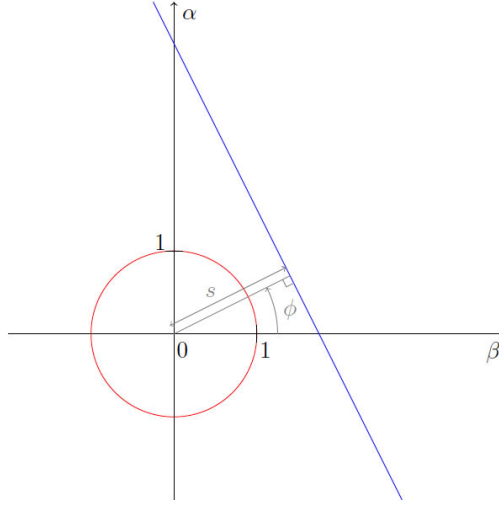
Figure 2. Polar coordinates used in the definition of the Radon transform in the usual (\beta, \alpha) -plane of DD variables. An integration line is defined by its (algebraic) distance s to the origin and the angle \phi between its normal and the abscissa axis.
