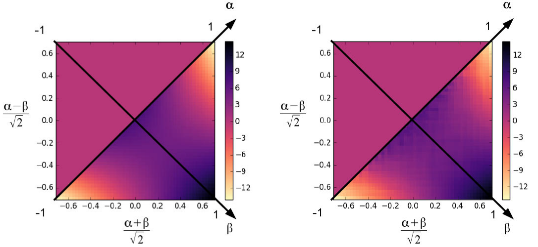
Figure 4. Left: Pion valence dressed-quark overlap GPD at t = 0 analytically computed from the DD in Eq. (16) in the Pobylitsa gauge. Right: Pion valence dressed-quark overlap GPD at t = 0 numerically computed from the DD resulting of the numerical Radon transform of the GPD restricted to the DGLAP region. The support for the parameters (\beta, \alpha) corresponds to a \pi/2 -rotated square with the two combinations (\alpha + \beta)/\sqrt{2} and (\alpha - \beta)/\sqrt{2} for the horizontal and vertical axes.
