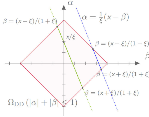
Figure 1. Integration lines defining a GPD at (x, \xi) in the (\beta, \alpha) -plane of DD variables.
