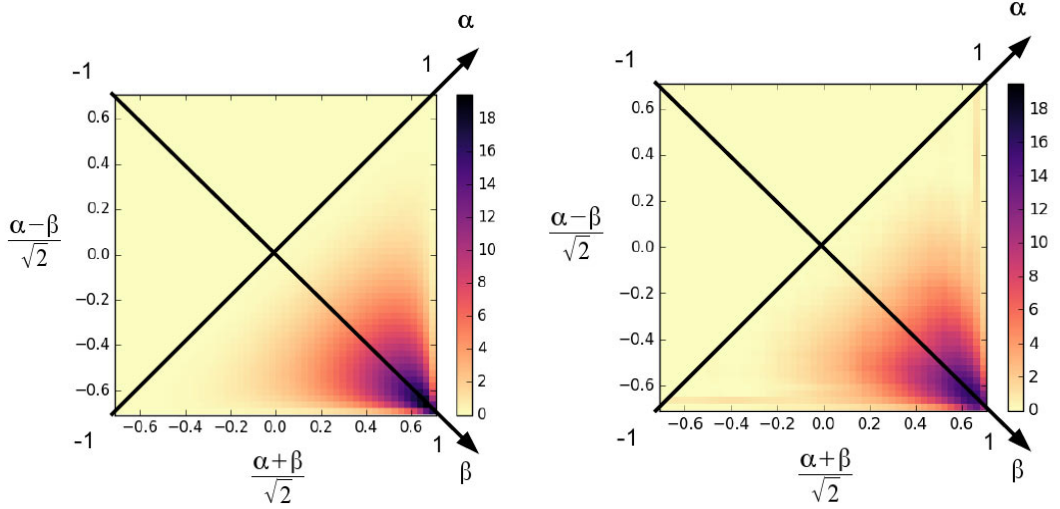
Figure 3. Left: Poblitsa-gauge DD for t = 0 obtained from the analytical expression Eq. (15). Right: DD resulting of the numerical inverse Radon transform of the associated GPD restricted to the DGLAP region. The support for the parameters (\beta, \alpha) corresponds to a \pi/2 -rotated square with the two combinations (\alpha + \beta)/\sqrt{2} and (\alpha - \beta)/\sqrt{2} for the horizontal and vertical axes.
