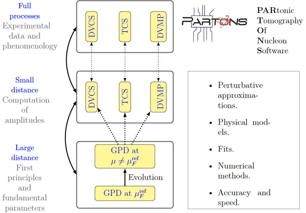
Figure 5. The architecture of the PARTONS code is designed to compute observables related to processes that can be factorized in short and large distance contributions.
