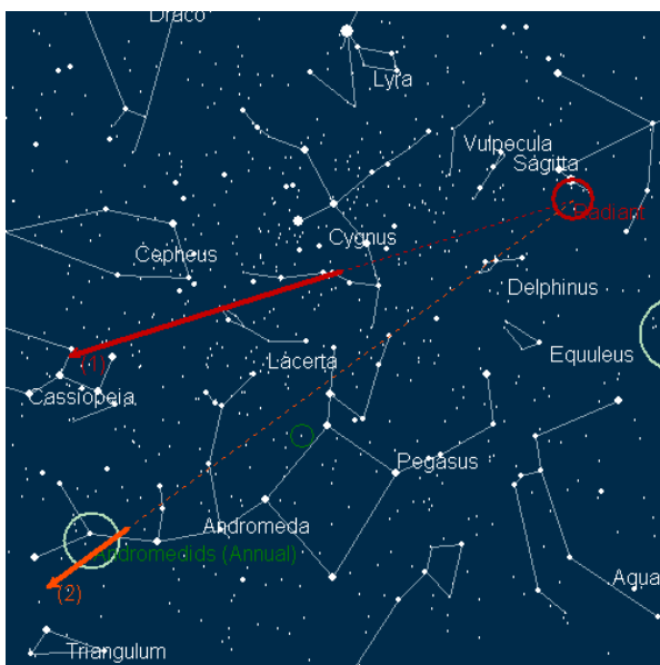
Figure 2. Radiant obtained by performing the astrometric calibration from the two meteor observing stations (1. Sevilla and 2. Arenosillo).
