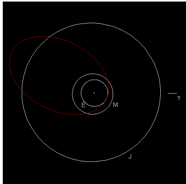
Figure 3. Heliocentric orbit of the SPMN131009 fireball. For comparison, the orbits of Jupiter, Mars and Earth are also shown..
