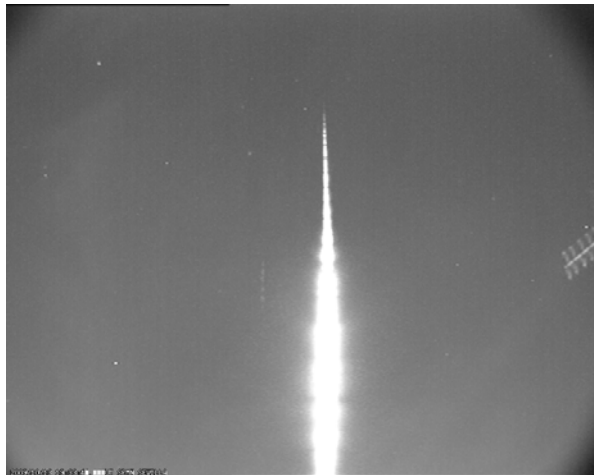
Figure 1. The Tarazona bolide (SPMN131009), with an absolute magnitude of -10 \pm 1 , imaged from Sevilla.
