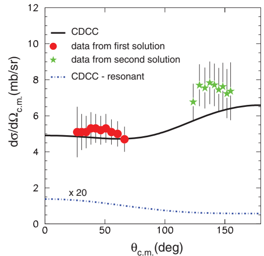
FIG. 5. Experimental and theoretical angular distributions, in the center-of-mass frame, for the ^7\text{Li} \rightarrow \alpha + t breakup for ^7\text{Li} incident on protons at 38.1 MeV. The experimental data, corresponding to the first kinematical solution, are denoted by filled red circles while the data corresponding to the second kinematical solution are denoted by green stars. The solid black line represents the result of the full CDCC calculation. The dot-dashed blue curve denotes the contribution of breakup via the 4.63 MeV 7/2^- resonance, multiplied by a factor of 20 in order to make it visible.
