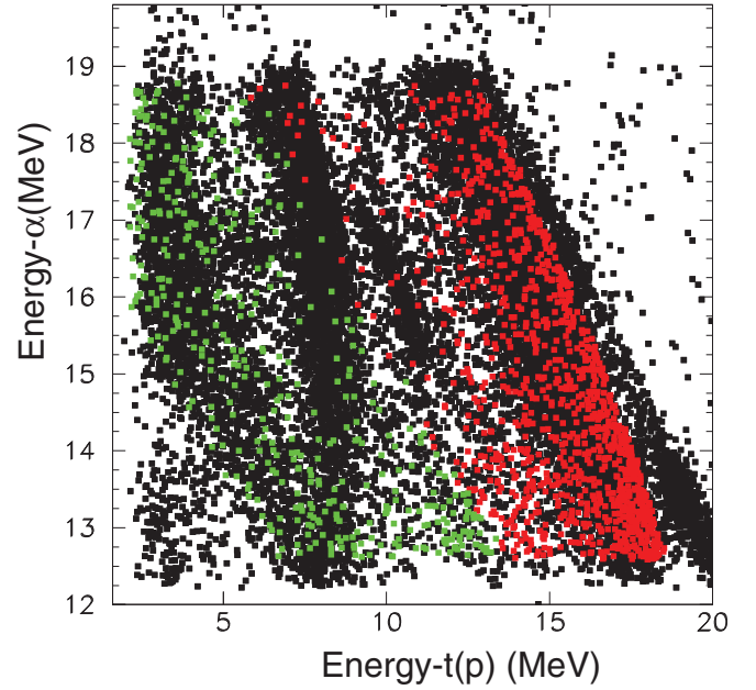
FIG. 2. Two dimensional energy spectrum determined at 38.1 MeV (5.44 MeV/nucleon) representing coincidence events of the two {}^7\text{Li} breakup fragments: \alpha energy versus triton or proton energy. The \alpha 's were recorded in the MAGNEX spectrometer over an angular range of \theta_{\text{lab}} = 0^\circ to 10^\circ , while the tritons and recoiling protons were registered in a silicon detector set at \theta_{\text{lab}} = 5^\circ . Superimposed on the experimental spectrum, denoted in black, are simulations of the first and second kinematical solutions, denoted as red and green dots respectively. The simulation represents in an excellent way the data in the left- and right-hand loci originating from \alpha 's in coincidence with tritons. The locus in the middle of the experimental (black) spectrum comes from coincidences of \alpha 's with the recoiling protons.
