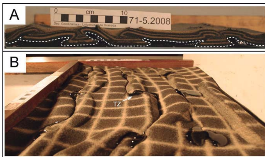
Fig. 3.- A. Cross-section representative of the structural style of the experimental wedges. (localized in the final stage of Model 71, Fig. 2B). Dashed white line: boundary between sand and silicone. B. Oblique view of the final stage of Model 71. TZ: Transfer Zone.
