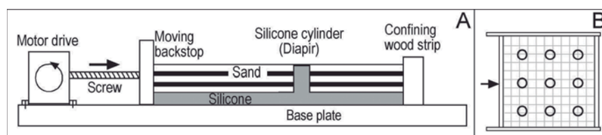
Fig. 1.- A. Simplified sketch of the experimental apparatus and model setting in cross section. B. Initial top surface of the model, with the position of the silicone cylinders (black circles).
