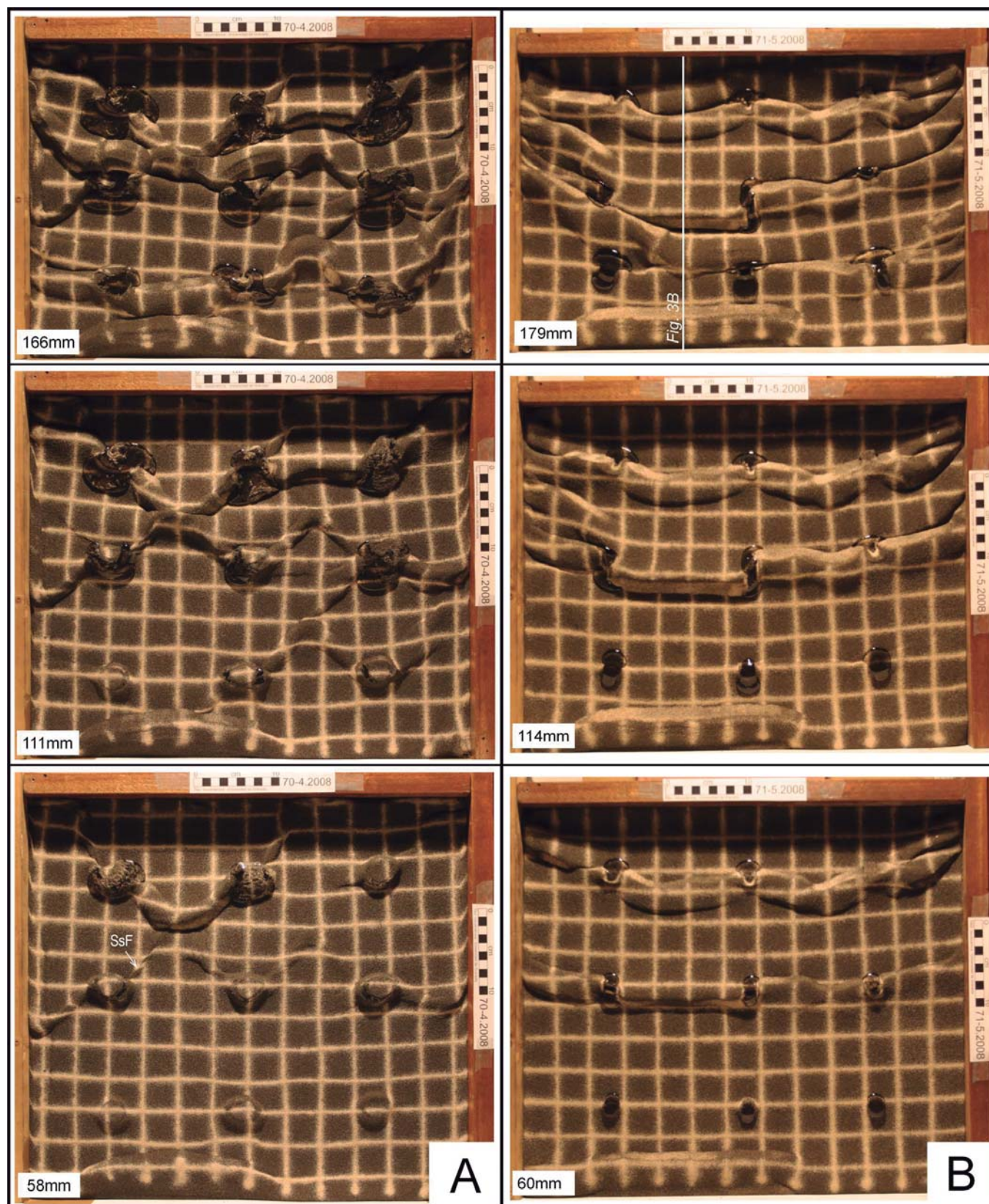
Fig. 2.- Photographs of map view of Models 70 (A) and 71 (B) for various amounts of shortening indicated as total movement of the backstop in millimetres. SsF: Strike-slip fault.
