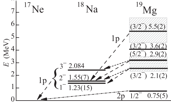
FIG. 1. The observed states in ^{19}\text{Mg} and ^{18}\text{Na} whose energies (in MeV) are shown relative to the respective 1p and 2p thresholds. The main and the minor ^{19}\text{Mg} \rightarrow ^{18}\text{Na} + p branches are indicated by dashed and dotted arrows, respectively. The spins and parities given in parentheses are tentative assignments. The energy of ^{18}\text{Na}(3^-) is taken from Ref. [10].
