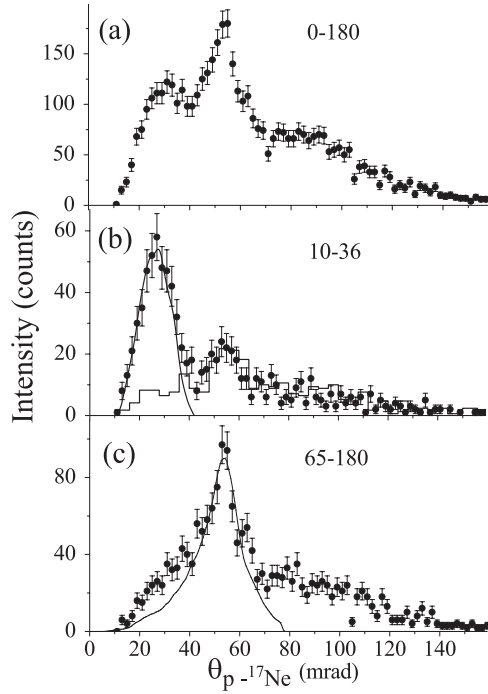
FIG. 3. (a) Angular p_1 - ^{17}\text{Ne} correlations (solid circles with statistical uncertainties) obtained from the measured ^{17}\text{Ne} + p + p data shown in Fig. 2(c) without imposing any gate condition. (b) Angular p_1 - ^{17}\text{Ne} distribution obtained from the same data by selecting the other proton angle, \theta_{p2-\text{Ne}} , within the range from 10 to 36 mrad, which corresponds to the assumed g.s. of ^{19}\text{Mg} . The solid curve represents the Monte Carlo simulation of the detector response to ^{19}\text{Mg}_{\text{g.s.}} \rightarrow ^{17}\text{Ne} + p + p with a 2p -decay energy of 0.75(5) MeV. The histogram represents the assumed background deduced from the data for a \theta_{p2-\text{Ne}} gate from 110 to 180 mrad; it contributes 15% to the peak at angles from 10 to 36 mrad. (c) Angular p_1 - ^{17}\text{Ne} distribution projected by choosing the \theta_{p2-\text{Ne}} gate from 65 to 180 mrad. The solid line is the simulation of the final-state interaction of protons with ^{17}\text{Ne} due to the 1.55-MeV resonance in ^{18}\text{Na} .
