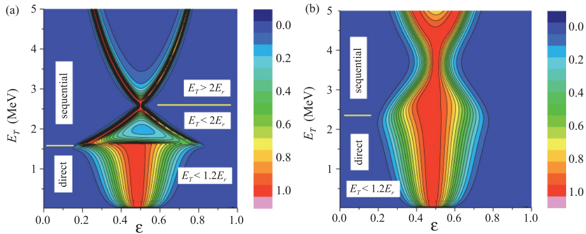
FIG. 5. (Color online) Intensity distributions of 2p decays from ^{19}\text{Mg} (arbitrary yields corresponding to the color scale shown on the right-hand side) as a function of the total 2p -decay energy E_T and the parameter \varepsilon \sim E_p/E_T . The distributions are calculated with a three-body model assuming a single resonance in the intermediate nucleus ^{18}\text{Na} with energy E_r and width \Gamma_r . (a) Decays by taking into account the g.s. of ^{18}\text{Na} at E_r = 1.23 MeV with \Gamma_r = 0.1 MeV. (b) Decays via the 1_2^- state in ^{18}\text{Na} at E_r = 2.03 MeV, \Gamma_r = 0.9 MeV [10].
