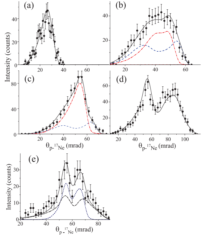
FIG. 4. (Color online) Angular p - ^{17}\text{Ne} correlations (solid circles with statistical uncertainties) selected from the ^{17}\text{Ne} + p + p data by choosing the arc gates (i–iv) shown in Fig. 2(c). (a) The 2p decay of the ^{19}\text{Mg} g.s. selected by gate (i), that is, the condition 20 < \rho < 45 mrad. The solid curve shows the best-fit simulation of the three-body model using a 2p -decay energy of Q_{2p} = 0.76(6) MeV. (b) The 2p decay of the ^{19}\text{Mg} “first-excited” state selected by the gate (ii), 50 < \rho < 65 mrad. The solid curve displays the simulation of the sequential 2p decay of the state at 2.14 MeV via two intermediate states in ^{18}\text{Na} , the g.s. at Q_{1p} = 1.23 MeV (dash-dotted line), and the 2^- state at 1.55 MeV (dashed line). (c) The 2p decay of the “second-excited” state in ^{19}\text{Mg} selected by gate (iii), 65 < \rho < 80 mrad. The solid line is the best-fit simulation of the sequential 2p decay of the ^{19}\text{Mg} state at 2.9 MeV via the 2^- and 3^- states in ^{18}\text{Na} (the dash-dotted and dashed curve, respectively). (d) The 2p decay of the suggested high-lying state in ^{19}\text{Mg} at Q_{2p} = 5.5 MeV selected by gate (iv), 90 < \rho < 115 mrad. The solid curve represents the best-fit simulation of the decay of this state by sequential 1p emission via ^{18}\text{Na}^*(2^-) . (e) Angular p - ^{17}\text{Ne} correlations selected by choosing the arc gate between areas (iii) and (iv) shown in Fig. 2(c), that is, the condition 80 < \rho < 90 mrad. The dashed curve shows the simulation of the sequential 2p decay of the suggested excited state in ^{19}\text{Mg} via ^{18}\text{Na}^*(2^-) , with the fitted values Q_{2p} = 3.6(2) MeV and \Gamma < 0.2 MeV. The dash-dotted curve represents the contribution due to the 2p decay of the neighboring ^{19}\text{Mg} state at Q_{2p} = 5.5 MeV. The solid curve is the sum fit.
