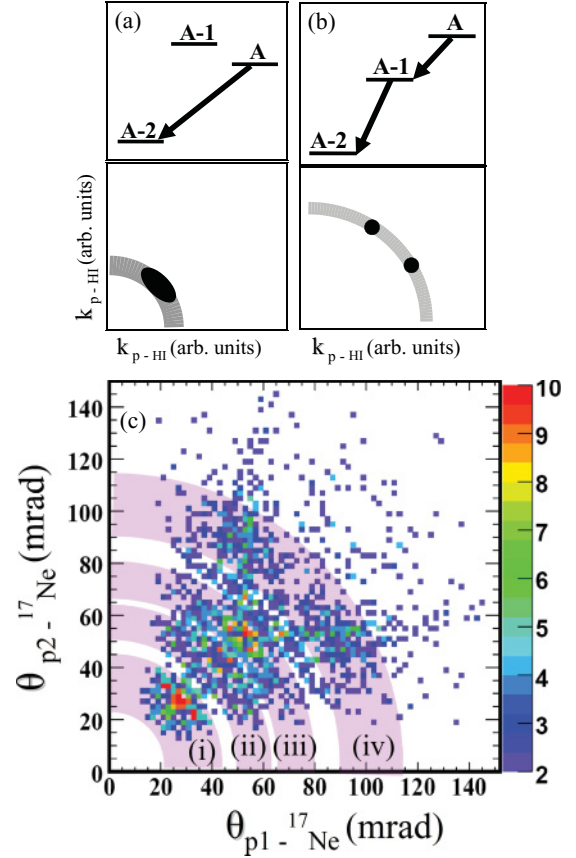
FIG. 2. (Color online) Schematic drawing of transverse momentum correlations k_{p1-\text{HI}}-k_{p2-\text{HI}} in panels (a), (b) expected for two alternative mechanisms of 2p decay (illustrated in the respective top panels) from a parent nucleus A to a daughter nucleus A-2 : (a) direct three-body decay or simultaneous 2p emission, (b) sequential emission of protons via a narrow intermediate state in nucleus A-1 . (c) Measured angular (p_1-^{17}\text{Ne}) - (p_2-^{17}\text{Ne}) correlations (color boxes with scale shown on the right-hand side). The shadowed arc areas (i-iv) (along \rho = \text{const} ) indicate locations of simultaneous or sequential 2p decays of the most intensively populated states in ^{19}\text{Mg} .
