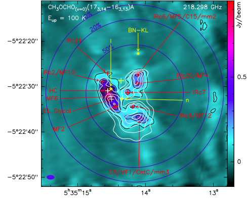
Fig. D.1. Continuum emission at 1.3 mm (color) overlaid with the HCOOCH 3 (white contours) emission at 218 298 MHz. Positions of the sources analysed in our Paper I are also given.
