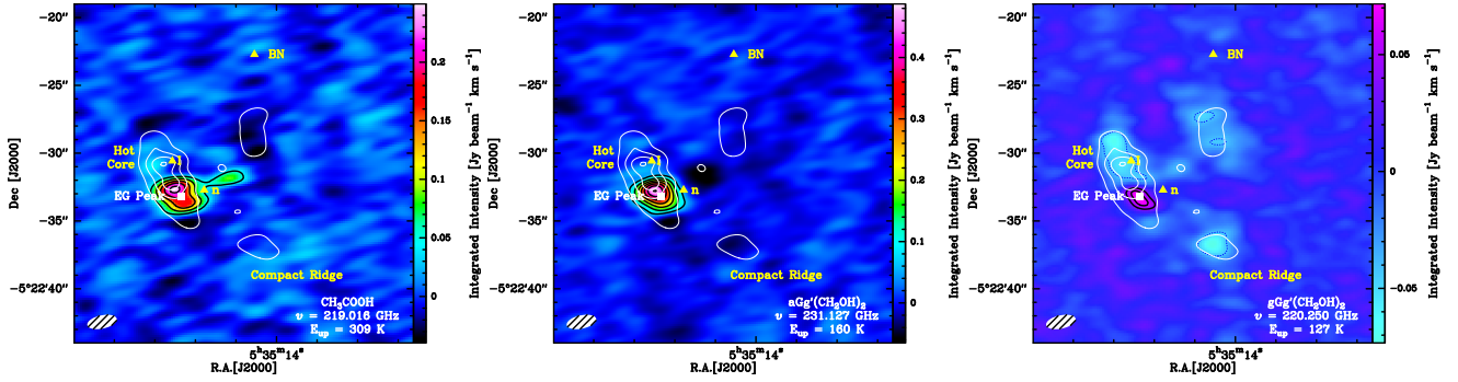
Fig. 1. Left panel: \text{CH}_3\text{COOH} integrated emission map at 219 016 MHz. The first contour and the level step are at 5\sigma (where 1\sigma = 9.3 \times 10^{-3} \text{ Jy beam}^{-1} \text{ km s}^{-1} ). Middle panel: \text{aGg}'(\text{CH}_2\text{OH})_2 integrated emission map at 231 127 MHz. The first contour and the level step are at 5\sigma (where 1\sigma = 1.4 \times 10^{-2} \text{ Jy beam}^{-1} \text{ km s}^{-1} ). Right panel: \text{gGg}'(\text{CH}_2\text{OH})_2 integrated emission map at 220 250 MHz. The contour levels are at -4 , 4 , and 6\sigma (where 1\sigma = 1 \times 10^{-2} \text{ Jy beam}^{-1} \text{ km s}^{-1} ). A narrow v_{\text{LSR}} interval (from 7 to 9 \text{km s}^{-1} ) has been selected to reduce confusion by nearby lines (see Sect. 3.3 and Appendix C). Positions of the radio source I, the BN object, and the IR source n (see Goddi et al. 2011) are indicated by yellow triangles. The white square indicates the position of the ethylene glycol peak ( \alpha_{\text{J2000}} = 05^{\text{h}}35^{\text{m}}14^{\text{s}}.47 , \delta_{\text{J2000}} = -05^{\circ}22'33''.17 ) by BD15. Finally, the continuum emission at 235 GHz is overlaid in white contours with a level step of 0.2 \text{ Jy beam}^{-1} (Paper I).
