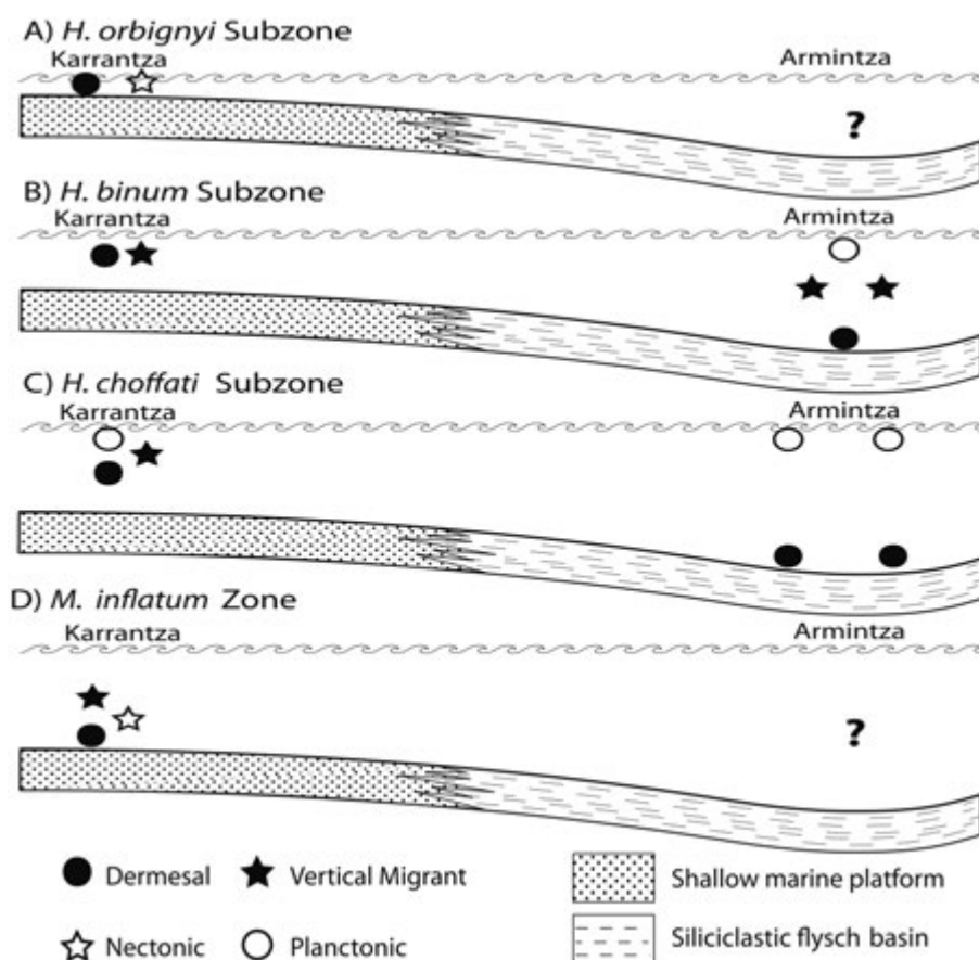
Fig. 3.- Interpretative bathymetric changes from H. orbigny to M. inflatum Biozones of Karrantza-Armintza. A) H. orbigny Subzone, shallow bathymetries. B) H. binum Subzone, vertical migrants indicate an increase of depth. C) H. choffati Subzone a planktonic specimen appear in Karrantza. D) M. inflatum Zone, increase of depth. Not to scale.
