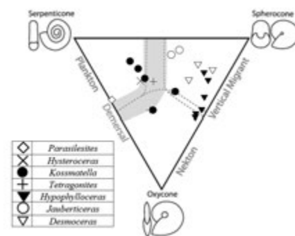
Fig. 2.- Ternary diagram in which ecomorphotypes have been established for the specimens belonging to H. binum Subzone in the study area (following Ritterbush and Bottjer, 2012).
