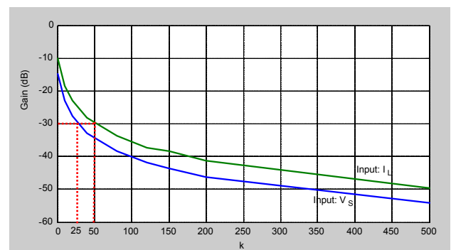
Fig. 3. Bode gain values versus k at frequency 250 \text{ Hz}
