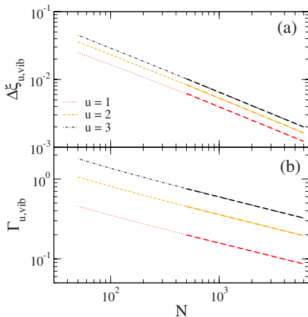
FIG. 18. (Color online) Double logarithm plot of the N dependence of \Delta\xi_{u,\text{vib}} , panel (a), and of \Gamma_{u,\text{vib}} , panel (b). These quantities are defined in Eqs. (73) and (71), respectively. The numerical calculation results are depicted with a dotted line, a dashed line, and a dotted-dashed line for u=1, 2, 3 , respectively. The fit to a power law was performed using the numerical results for N=500-6000 and the result is depicted using thicker dashed lines in the plot.
