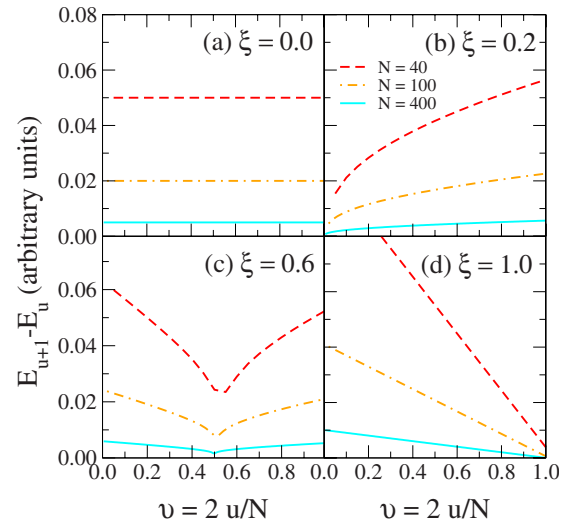
FIG. 5. (Color online) Birge-Sponer or anharmonicity plot where the energy difference E_{u+1} - E_u is plotted as a function of \nu=2u/N for N=40, 100, 400 . The values of the control parameter are \xi=0.0, 0.2, 0.6 , and 1.0 for panels (a), (b), (c), and (d), respectively. Energy units are arbitrary and the energy scale \epsilon=1 .
