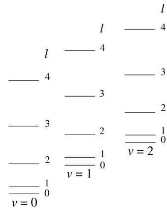
FIG. 2. Energy spectrum of the two-dimensional displaced oscillator associated to chain (II), Eq. (25), with parameters N=10 , \beta=0.5 , and A=-0.1 . The first three vibrational bands, v=0, 1, 2 , with l \leq 4 are shown. Levels with l \neq 0 are doubly degenerate, \pm l .
