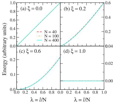
FIG. 6. (Color online) Rotational excitation plot, where the v=0 rotational band energies are plotted as a function of \lambda=l/N for N=40, 100, 400 . The values of the control parameter are \xi=0.0, 0.2, 0.6 , and 1.0 for panels (a), (b), (c), and (d), respectively. Energy units are arbitrary and the energy scale \epsilon=1 . Ground-state energy has been set to zero.
