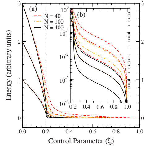
FIG. 19. (Color online) Panel (a), correlation energy diagram that shows the rotational excitation pattern for the l=1, 2 , and 3 states of the lowest u=0 band and N=40, 100, 400 . The energy units are arbitrary and the scale \epsilon=1 . Ground-state l=0 energies have been set to zero and the critical value of the control parameter \xi_c=0.2 has been marked with a vertical dotted-dashed line. Panel (b) depicts the behavior for \xi > 0.2 in logarithmic scale.
