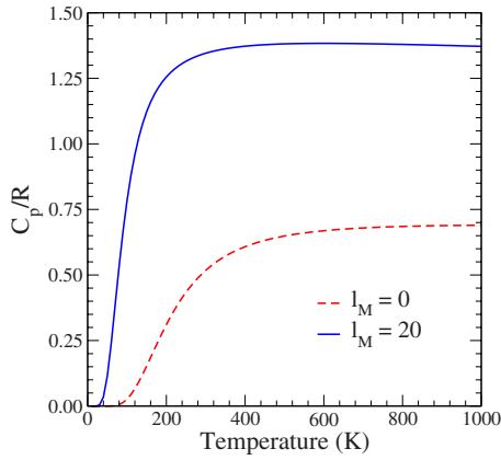
FIG. 25. (Color online) Heat capacity \gamma = C_p/R associated to the H-C-NO bending degree of freedom ( \nu_5 ) of fulminic acid (HCNO). The dashed (red) line corresponds to the purely vibrational calculation, l=0 , while the full (blue) line combines vibrations and rotations up to l_M=20 , where convergence in calculations occurs for the considered temperature interval.
