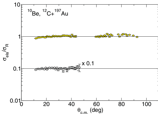
FIG. 2. (Color online) Elastic scattering angular distributions for the ^{10}\text{Be} + ^{197}\text{Au} system multiplied by 0.1 (open circles) and ^{12}\text{C} + ^{197}\text{Au} (filled circles). See text for details.
