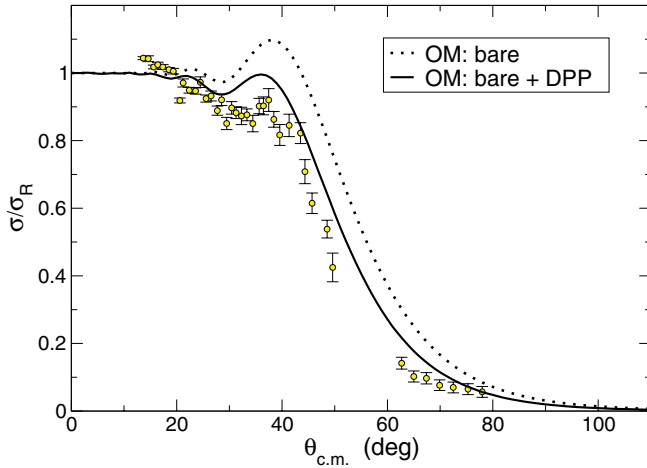
FIG. 8. (Color online) Elastic scattering angular distribution for the ^{11}\text{Be}+^{64}\text{Zn} system (symbols). The dotted line is the OM calculation performed with the bare interaction alone, and the solid line is the OM calculation adding the Coulomb DPP to the bare potential. See text for details.
