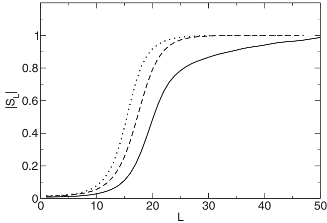
FIG. 6. Modulus of the elastic S matrix as a function of the angular momentum for ^9\text{Be}+^{64}\text{Zn} (dotted line), ^{10}\text{Be}+^{64}\text{Zn} (dashed line), and ^{11}\text{Be}+^{64}\text{Zn} (solid line).
