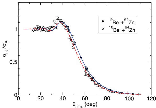
FIG. 3. (Color online) Elastic scattering angular distribution for the ^9\text{Be} + ^{64}\text{Zn} system (filled symbols) and ^{10}\text{Be} + ^{64}\text{Zn} system (open symbols). Lines represent the results of the OM analysis (see text for details).
