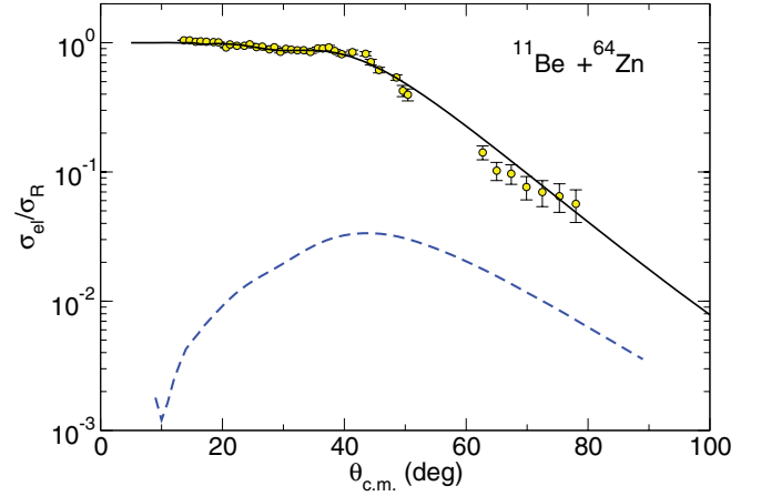
FIG. 7. (Color online) Measured quasielastic angular distribution for ^{11}\text{Be}+^{64}\text{Zn} (symbols), compared with an OM fit of the data (solid line) and a DWBA calculation (dashed line) for the inelastic scattering to the first excited state of ^{11}\text{Be} .
