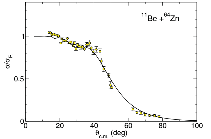
FIG. 4. (Color online) Elastic scattering angular distribution for the ^{11}\text{Be} + ^{64}\text{Zn} system. The solid line represents the results of the OM analysis (see text for details).
