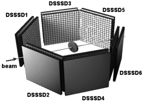
FIG. 1. Experimental setup used for the ^{10,11}\text{Be} + ^{64}\text{Zn} experiment.
