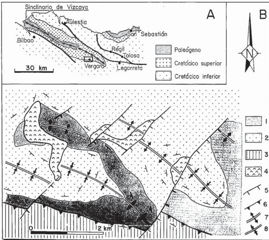
Fig. 1.-A: Location of the area studied in the northern portion of the Basque-Cantabrian Basin. B: Simplified geological map of the area studied. 1) Volcanic rocks (Middle to Upper Cretaceous), 2) marls and limestones (Middle to Upper Cretaceous), 3) black shales and sandstones (Lower and Middle Cretaceous), 4) evaporitic rocks (Triassic) with blocks of scapolite-bearing marbles, 5) normal fault, 6) reverse fault, 7) anticline, and 8) syncline. Outcrops of evaporites are found in the core of an anticline cut off by transversal faults. Most of the largest outcrop of triassic rocks is hidden below the town of Vergara.
