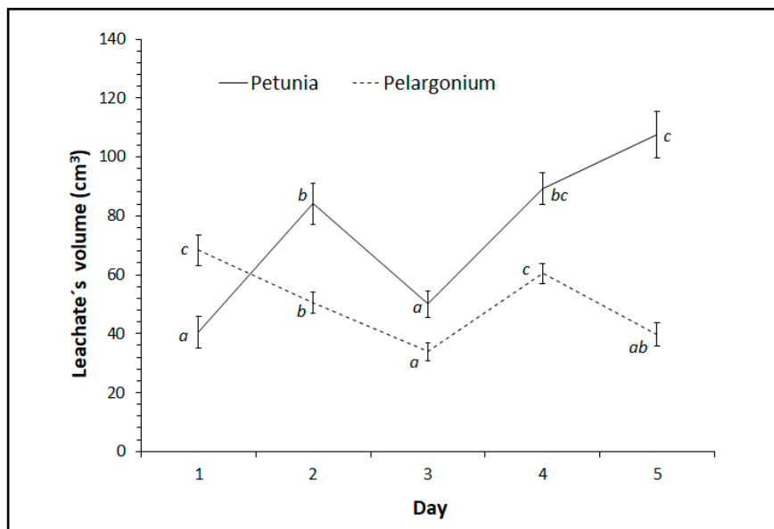
Figure 2. Leachate's volume (cm 3 ) of petunia and geranium grown in mixtures with different proportions of peat-based substrate (S), vermicompost (V) and biochar (B), (S:V:B). For each species letters show significant differences among sampling dates ( p < 0.05 ). Huelva, ETSI, 2017.
