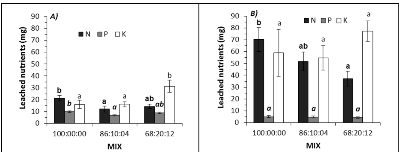
Figure 3. Total amount of nutrient leached by containers taken into account the five sample days. Letters show significant differences between substrates studied ( p < 0.05 ), Tukey-HSD test. (A) Petunia , (B) Pelargonium . Huelva, ETSI, 2017.
