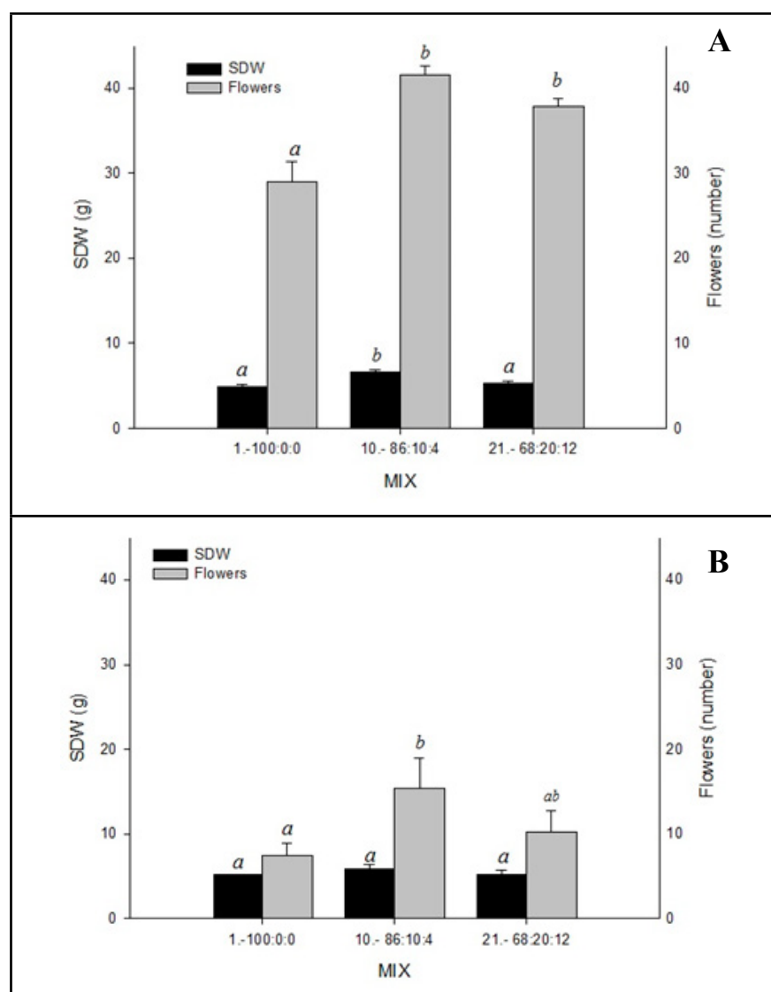
Figure 1. Shoot dry weight (SDW, g) and flower production number of petunia (A) and pelargonium (B) grown in mixtures with different proportions of peat-based substrate (S), vermicompost (V) and biochar (B) (S:V:B). Letters show significant differences between substrates studied ( p < 0.05 ). (Tukey-HSD test for SDW both species, and for flowers in Petunia; T3-Dunnet test for flowers in Pelargonium). Columbus, OSU, 2016.
