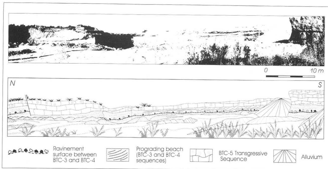
Fig. 4 - El Cuervo Section. The internal arrangement of the upper part of the BTC can be observed. See text for explanation.
