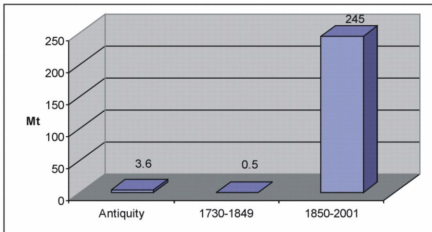
Figure 10. Sulphide production (run-of-mine ore) in the Río Tinto area throughout history.
