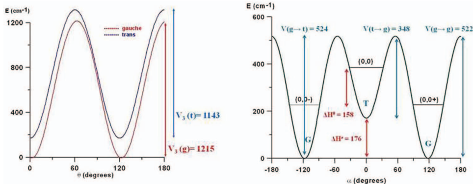
FIG. 2. Torsional energy barriers of ETSH calculated at the CCSD(T)/aug-cc-pVTZ level: (left) methyl torsion barriers; (right) thiol torsion barriers.
