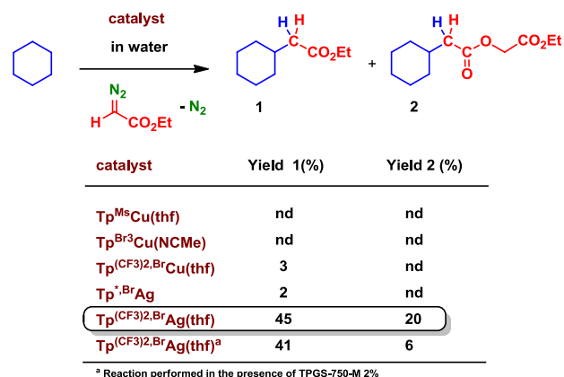
Scheme 3. Functionalization of cyclohexane in water
