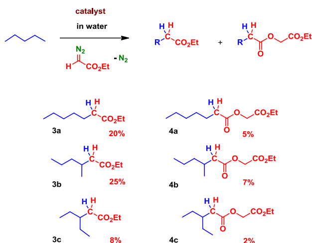
Scheme 4. Functionalization of pentane in water (yields based on EDA).
