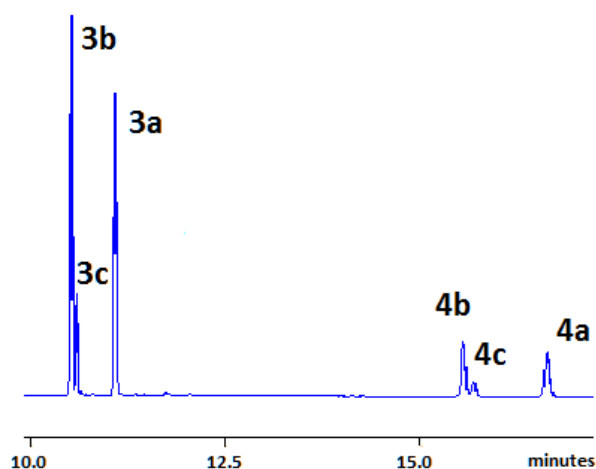
Figure 1. GC trace of the reaction mixture of the functionalization of pentane
