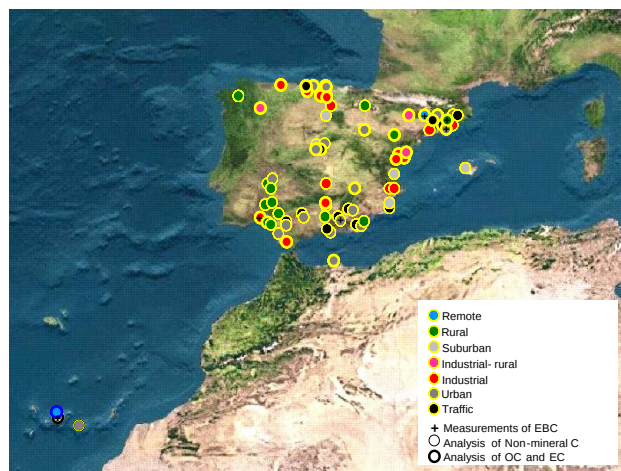
Fig. 1. Location of the monitoring stations across mainland Spain, the Balearic and Canary Archipelagos and the Spanish northern African territories from where data on nmC, OC, EC and EBC were obtained during the period 1999–2011.
