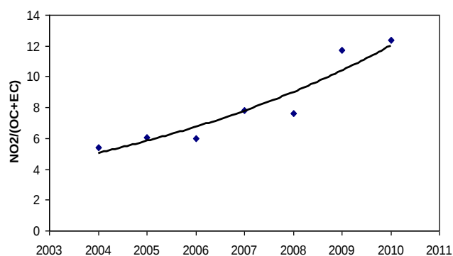
Fig. 10. NO 2 /(OC + EC) rates as obtained from OC + EC measurements in PM 2.5 performed at the Barcelona urban background site and from NO 2 measured at another urban background site in Barcelona (Ciutadella) by the Air Quality Department of the Autonomous Region of Catalonia.
