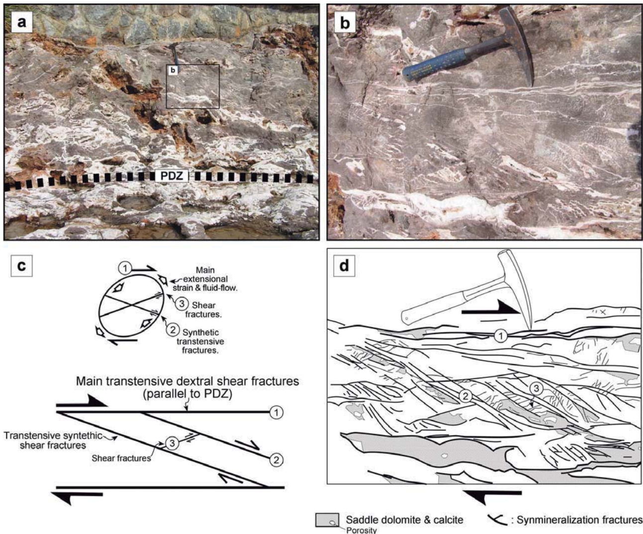
Fig. 2.- San Martín beach dolomites . A: Oblique view of dolomitized transverse fracture zone (PDZ: Principal displacement zone). B: Transverse shear fractures with saddle dolomite (D 2 ) infill. C: Proposed structural sketch to explain the fracturation and mineralization pattern. D: Synmineralization fracture sketch of «B» photograph.
